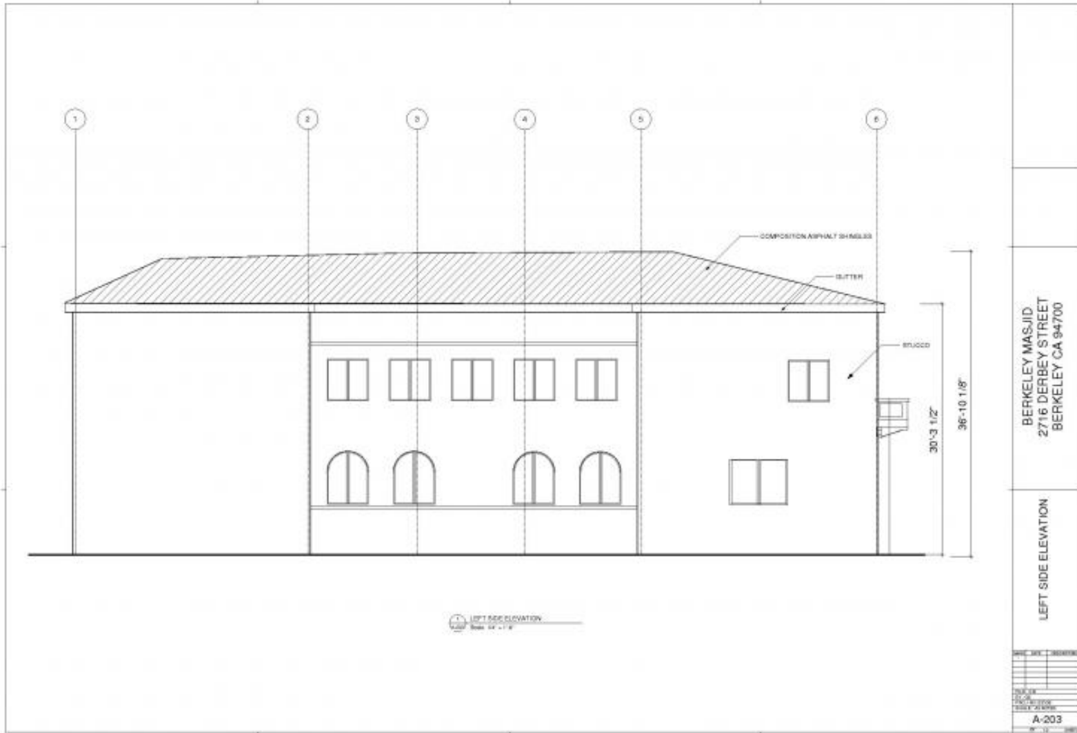
EAST ELEVATION
