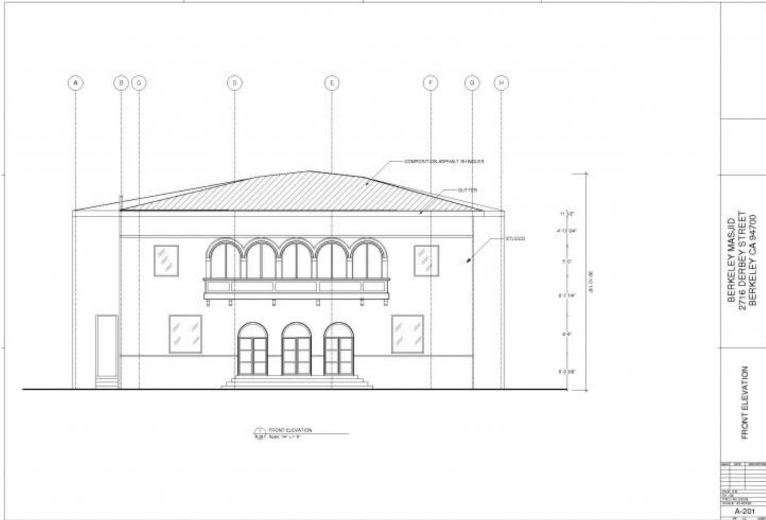
NORTH (FRONT) FAÇADE
