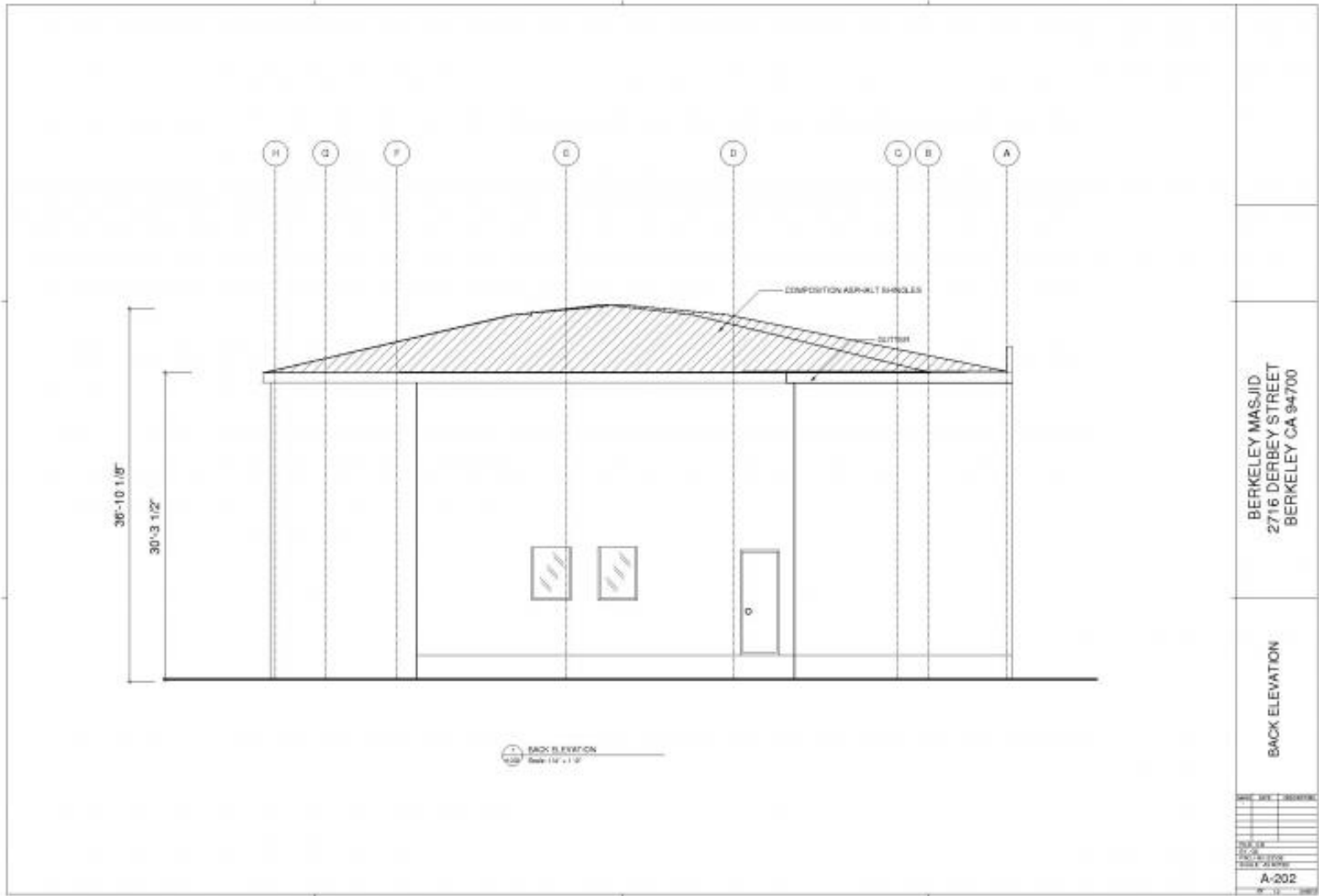
SOUTH (REAR) ELEVATION
